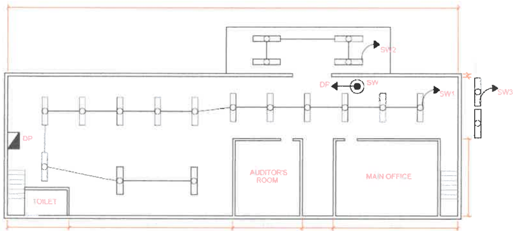
EXISTING G/F 1 GROUND FLOOR PLAN A1/00 SCALE 1:150 METERS
